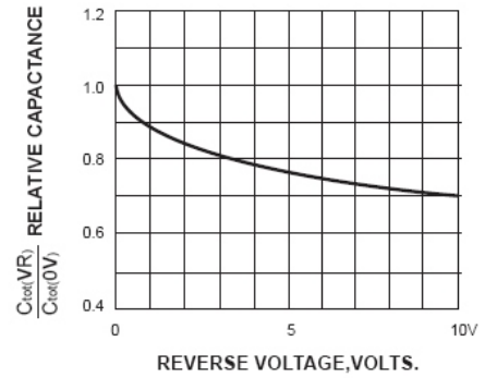
FIG. 4-RELATIVE CAPACTANCE VERSUS REVERSE VOLTAGE
