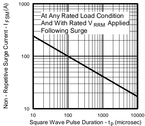
Fig.7 Max. Non-Replicative Surge Current (Per Leg)
